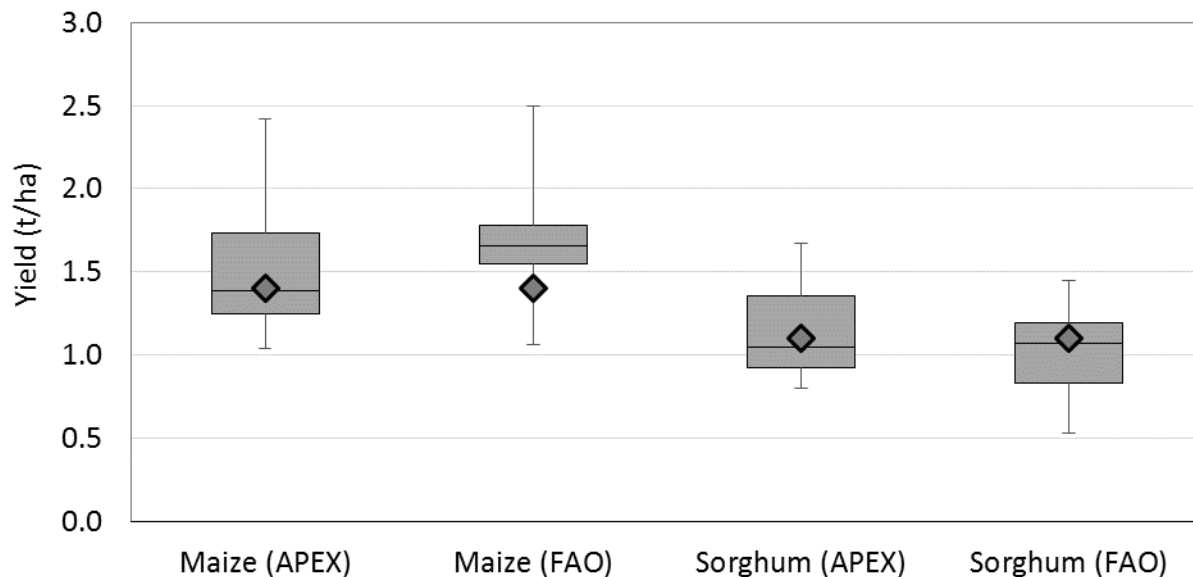
Figure 7: Comparison of APEX vs. FAOSTAT maize and sorghum yields from 1983 to 2013, with SPAM crop yield for year 2005 represented by a diamond.
