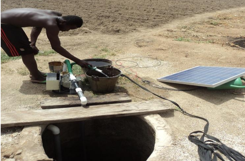
Solar pump installed in Ghana. (Source: Bern University of Applied Sciences, 2013)
