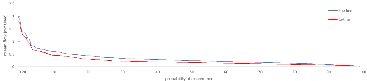
Figure 13. Flow duration curve for the monthly stream flow at the outlet of the Nimbasinia watershed in the baseline scenario and SSI (ex ante) scenario.
