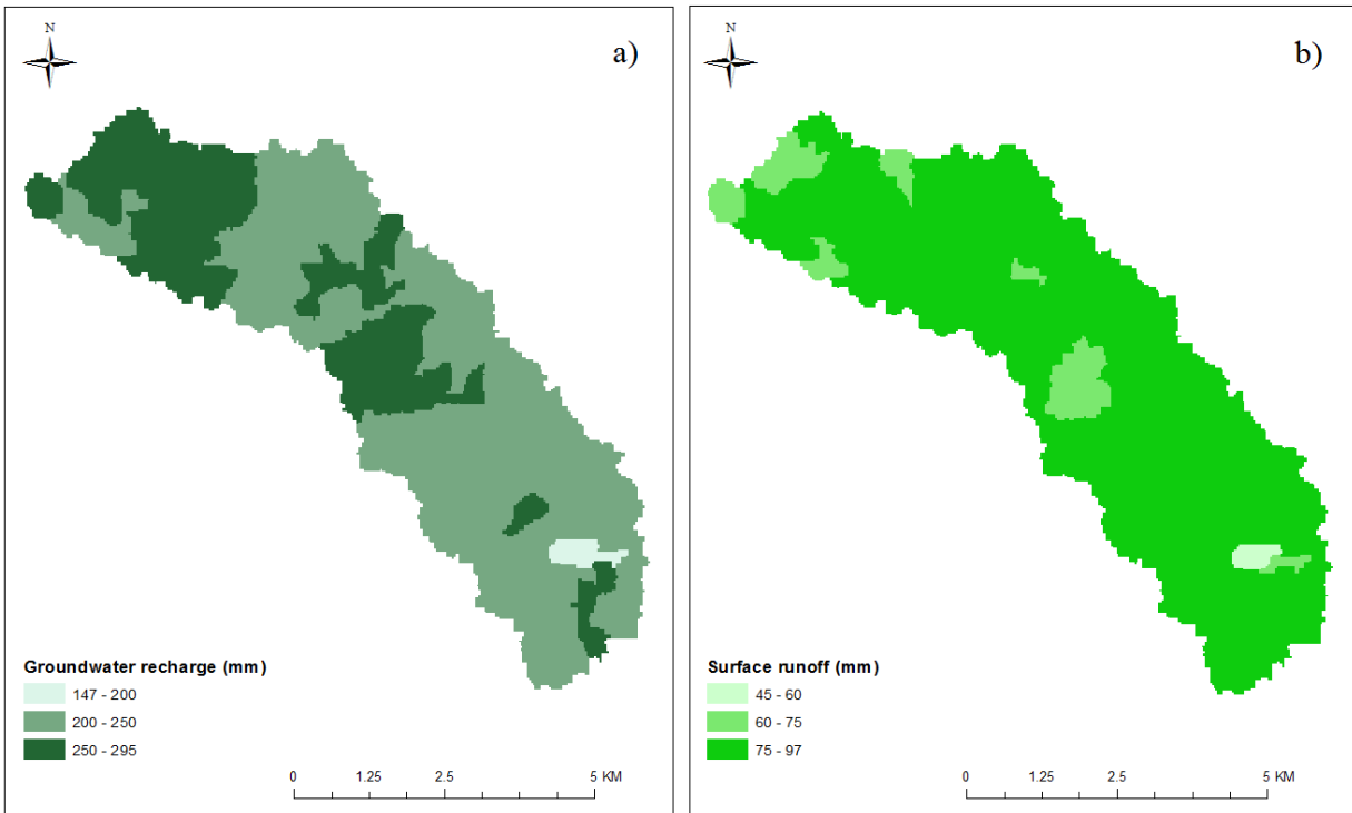
Figure 8. Water resources potential in the Nimbasinia watershed: a) average annual groundwater recharge; and b) average annual surface runoff.
